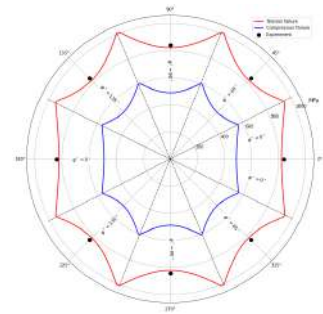
Figure 1: Failure envelope for IM7/8552 carbon-epoxy laminates
